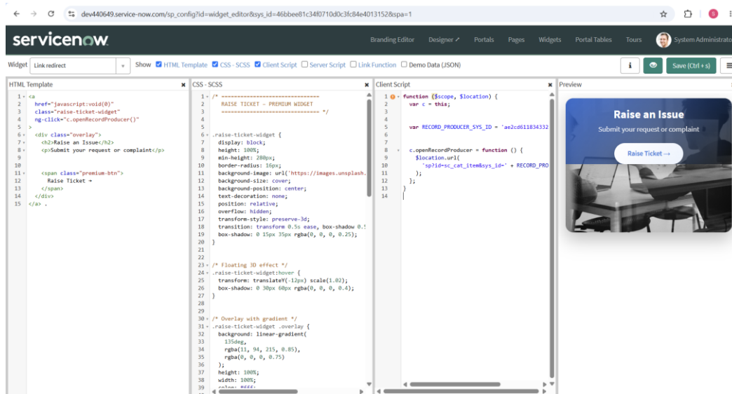
Figure 2. Custom Raise an Issue Widget and Navigation Configuration
